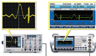
Direct Waveform Reconstruction from the GDS-2000 Series
