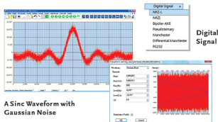
Gaussian Noise
