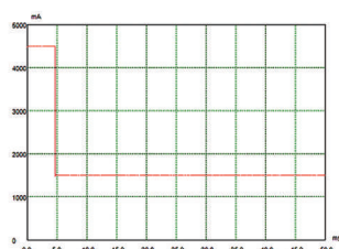
Pulse Current Measurement
