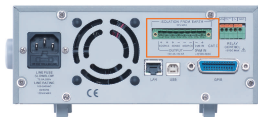
Rear Panel of PPH-1503 (Output Terminal)
