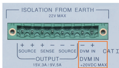
Rear Panel of the PPH-1503
