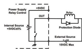
External Power Source
