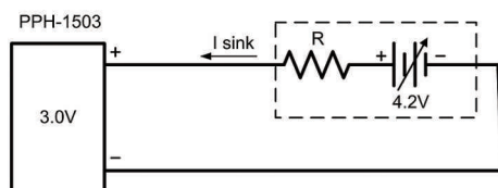
Current Sink Connection
