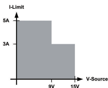
Dual Range Operation
