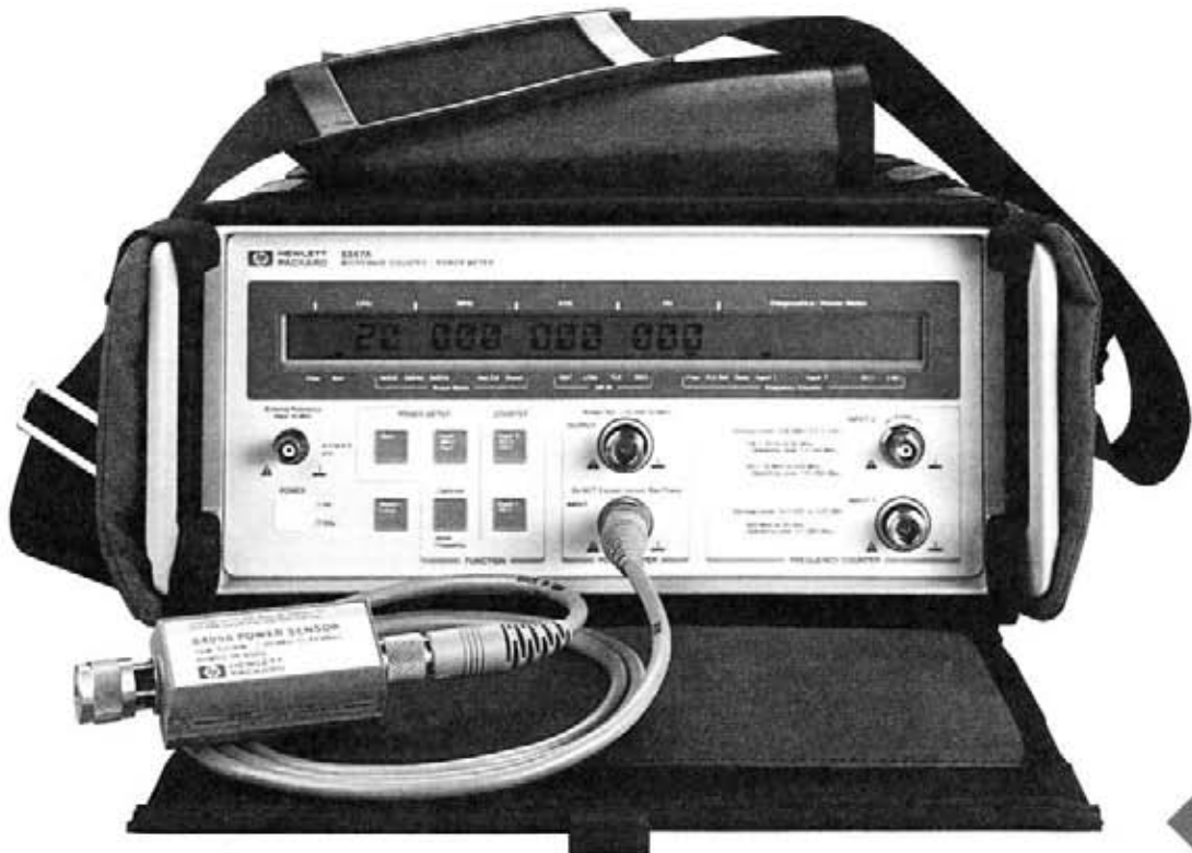
HP 5347A portable microwave counter/power meter. (Shown with Option 803, HP 8485A power sensor, and Option 070 soft carrying case.)
