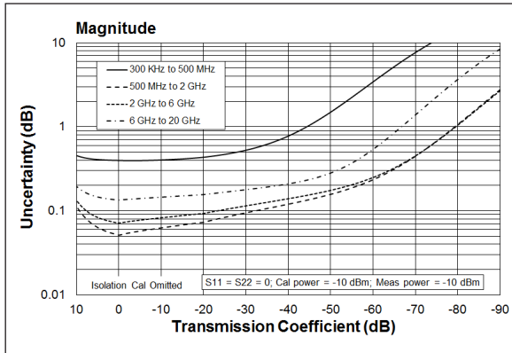
Transmission uncertainty (specification)
