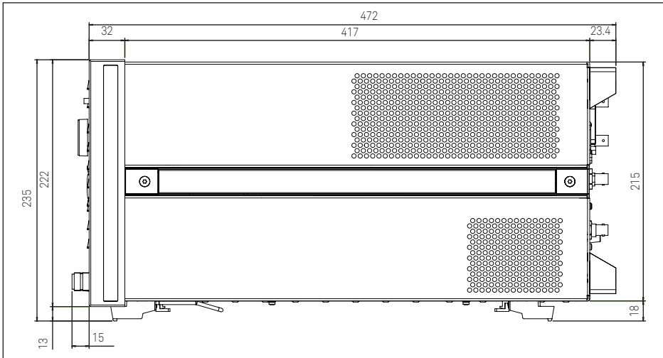
Figure 8. Dimensions (side view, E5071C Option 230/235/240/245/260/265/280/285/430/435/440/445/460/465/480/485, in millimeters)
