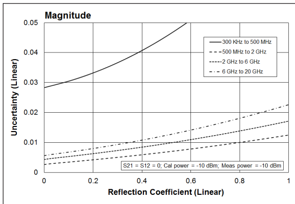
Reflection uncertainty (specification)
