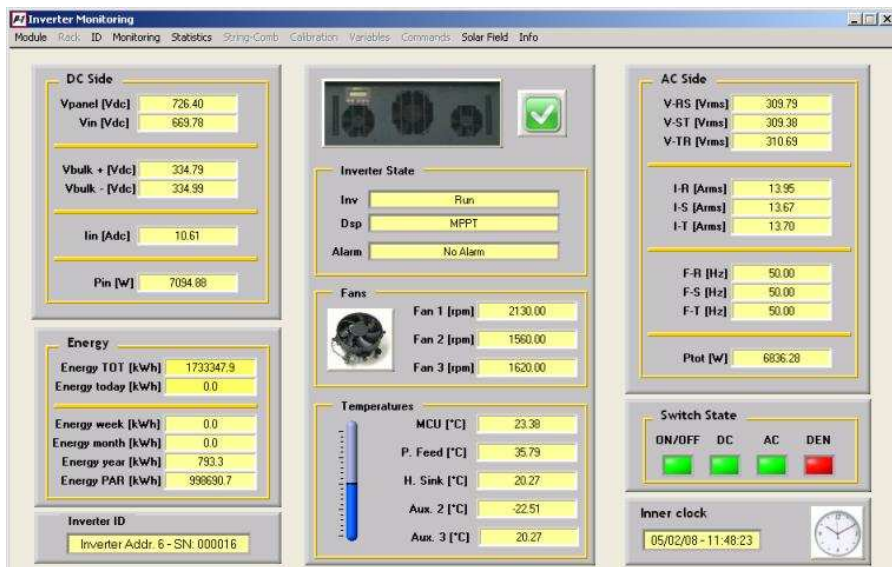
Figura 15-10: Inverter Monitoring
