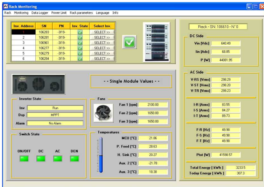
Figura 15-11: Rack Monitoring
