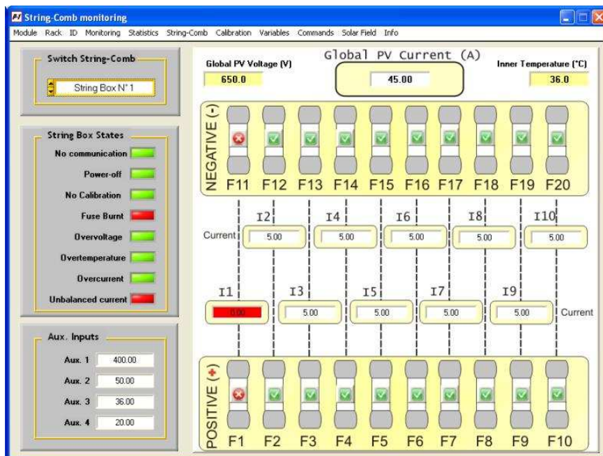
Figura 15-17: StringComb monitoring
