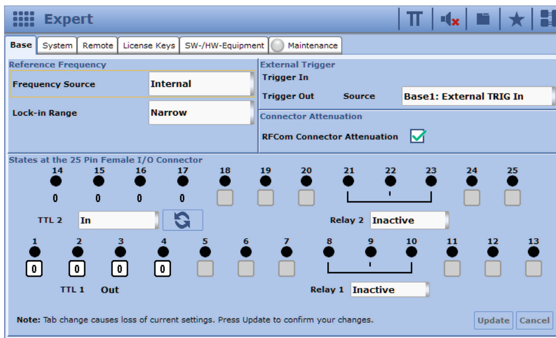
External connection via relays and TTL I/Os
