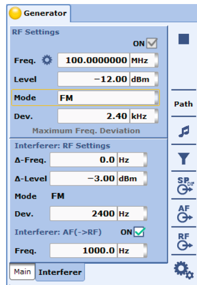
Frequency modulation with an integrated interfering signal
